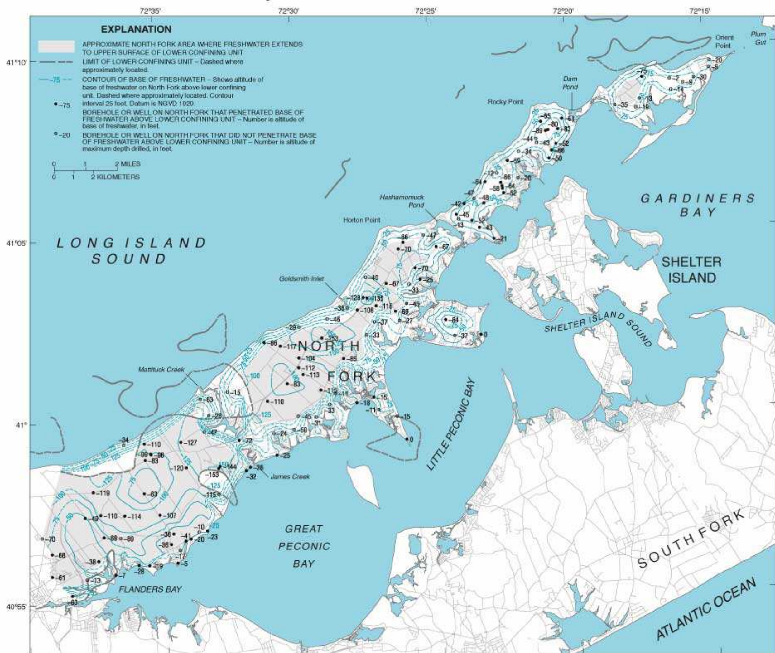
B. Altitude of base of freshwater above lower confining unit
