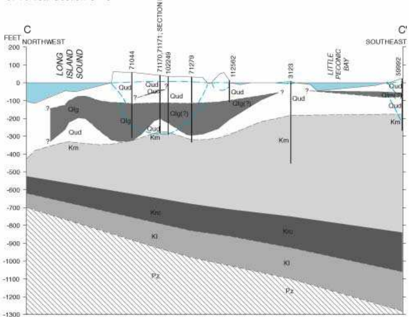
C. Vertical Section C - C'
