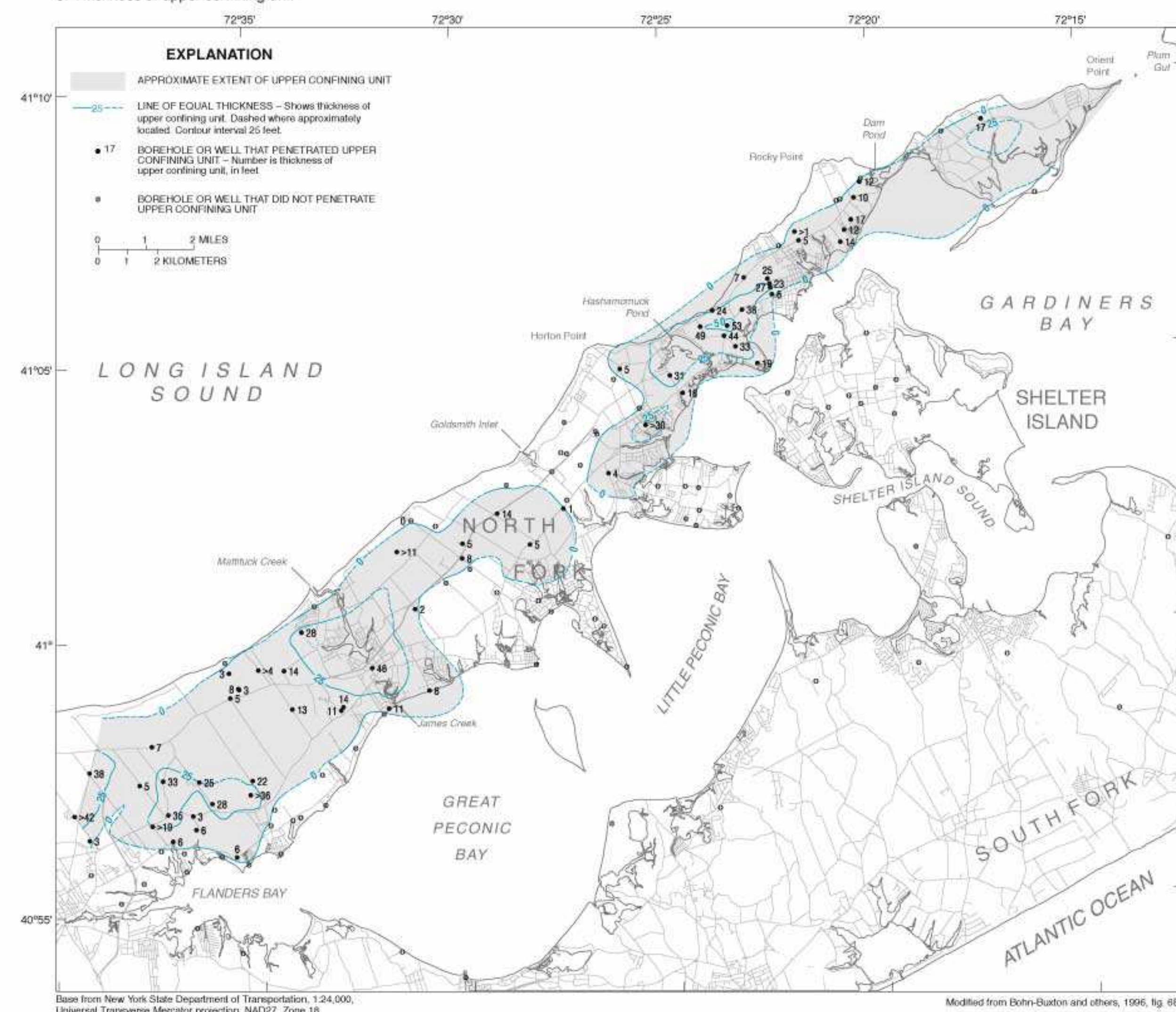
C. Thickness of upper confining unit
