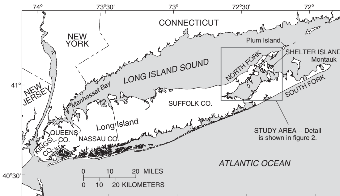
Figure 1. Principal geographic features of North Fork study area in eastern Suffolk County, Long Island, N.Y.
