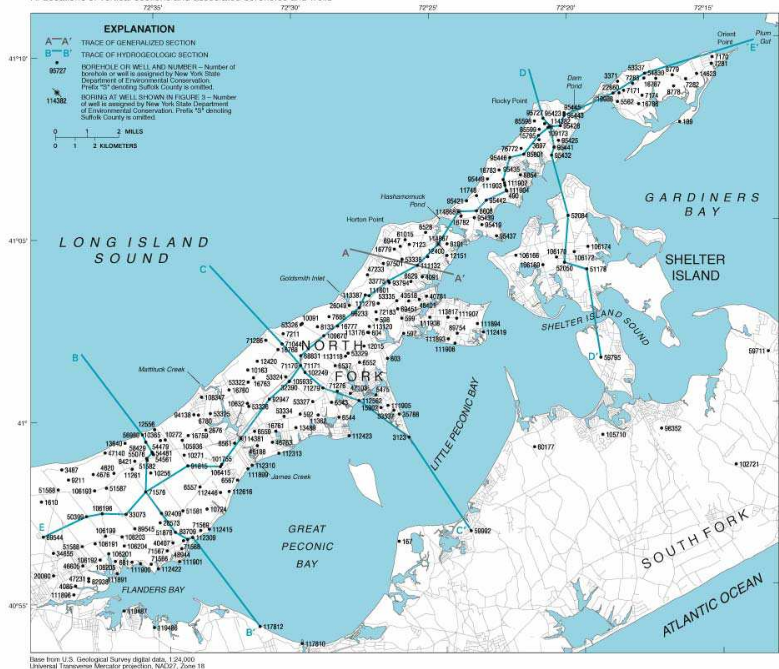
A. Locations of vertical sections and associated boreholes and wells
