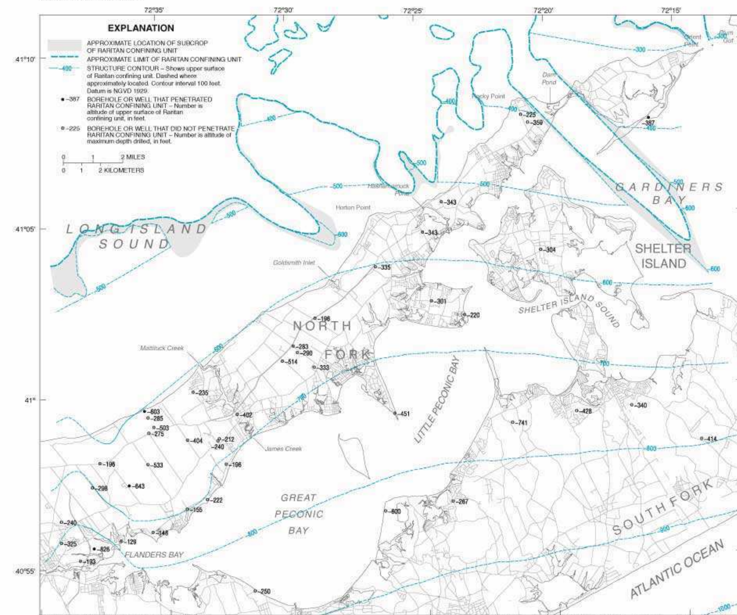
C. Raritan confining unit
