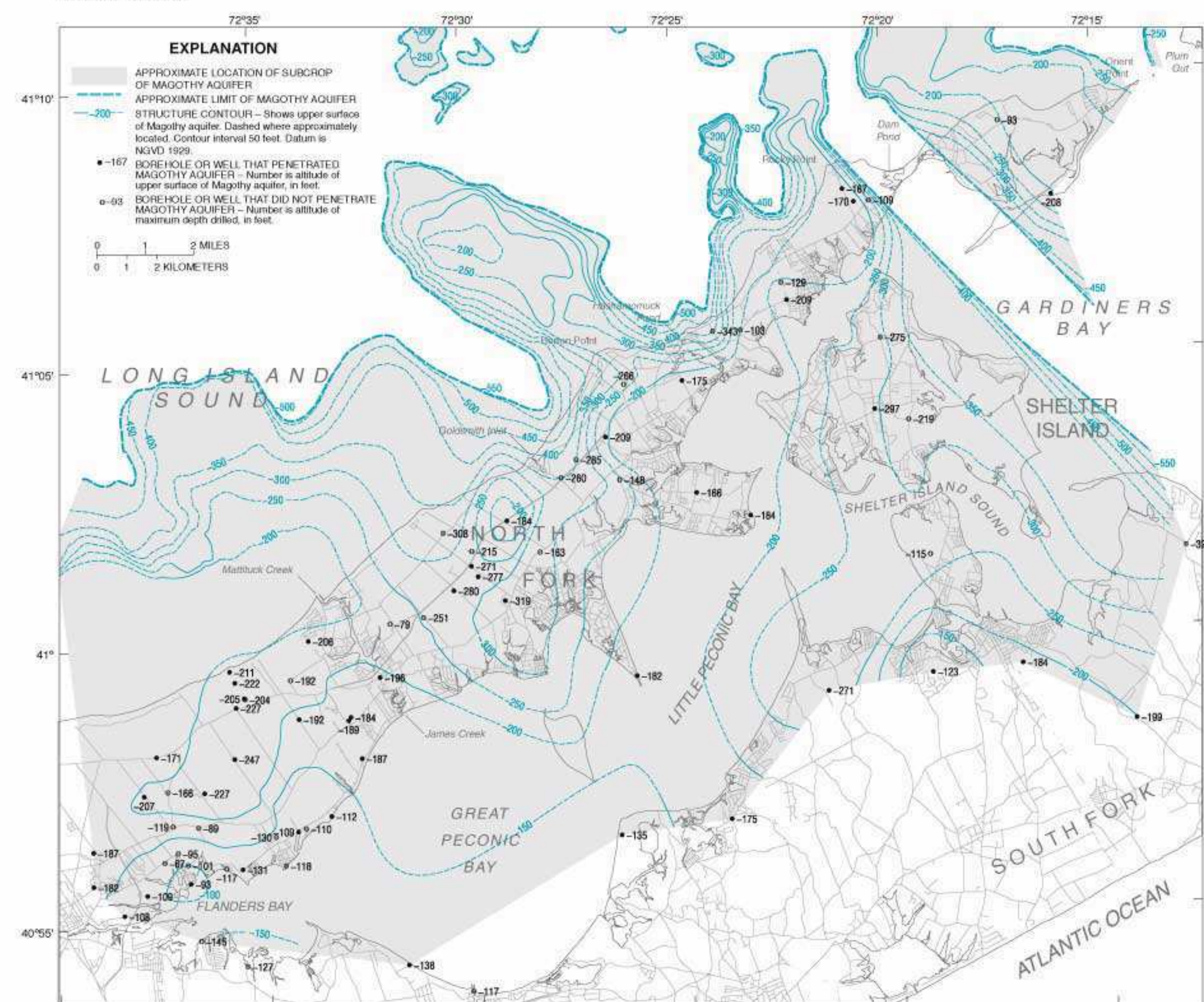
D. Magothy aquifer
