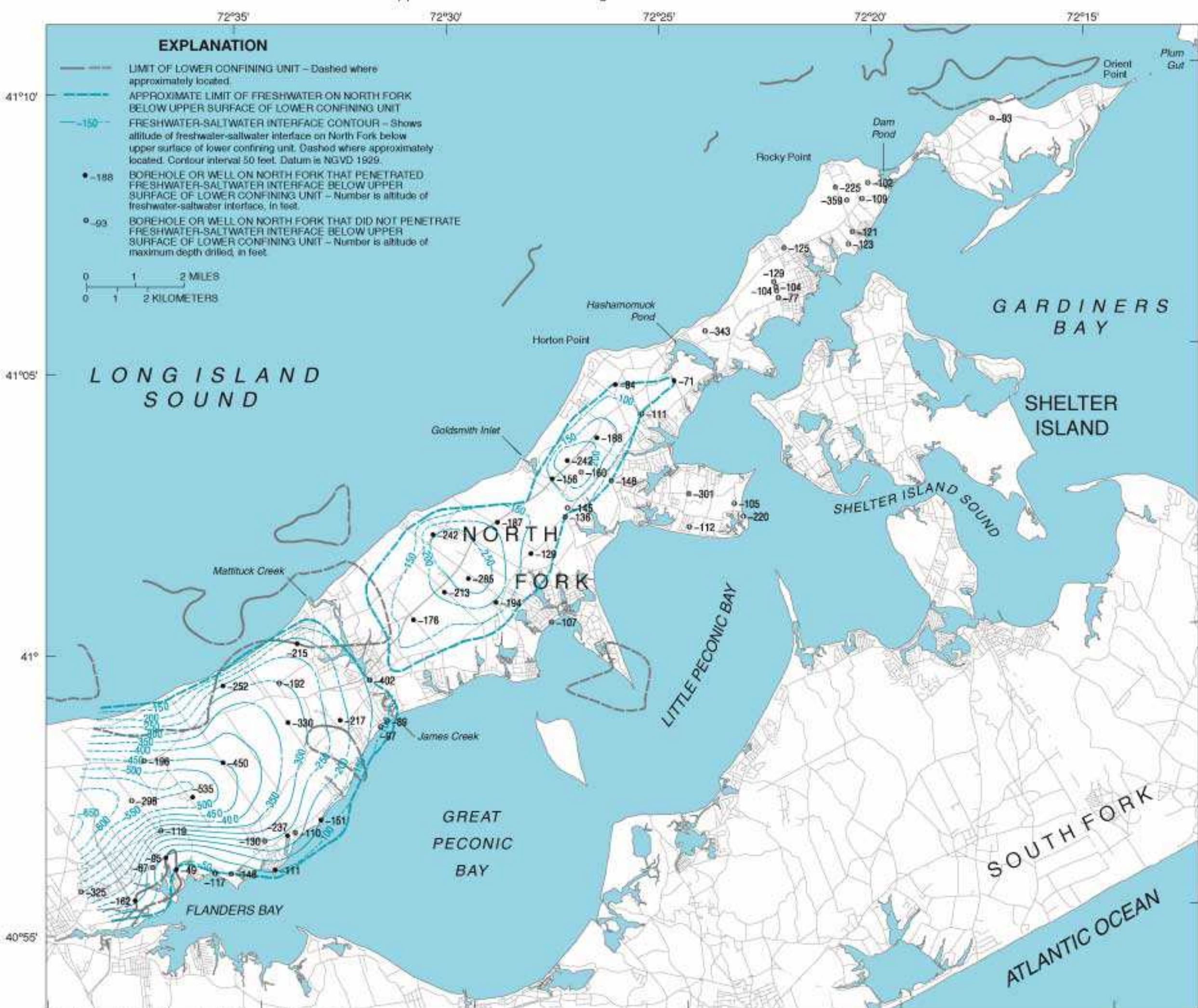
C. Altitude of freshwater-saltwater interface below upper surface of lower confining unit
