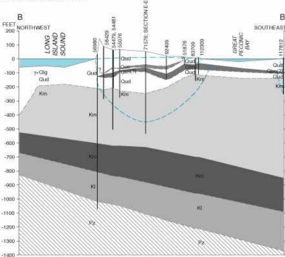
B. Vertical Section B - B'
