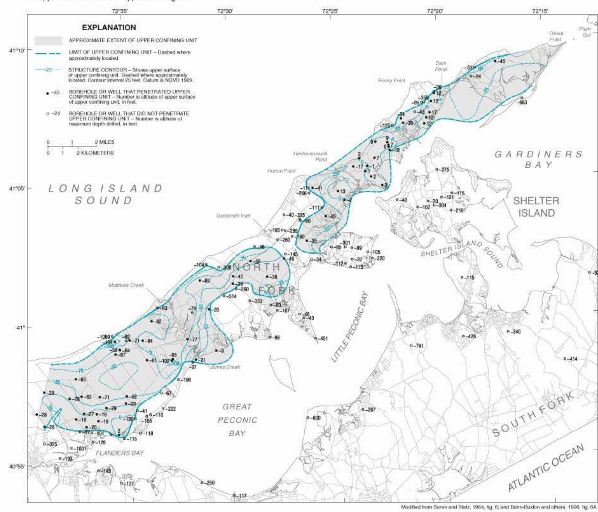
D. Upper-surface altitude of upper confining unit
