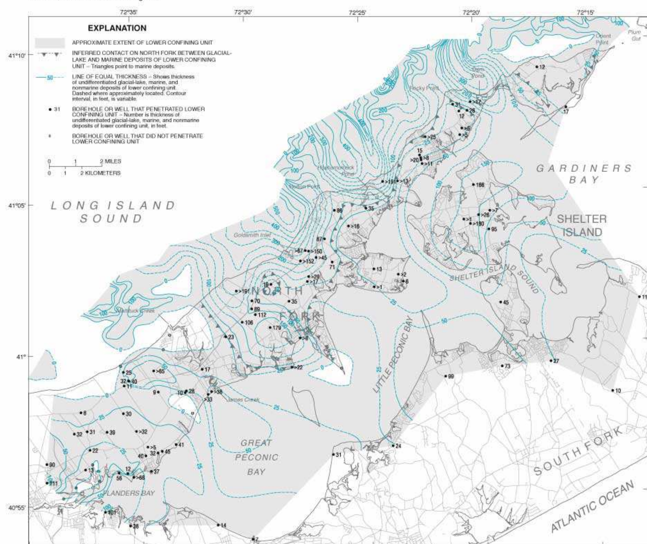
A. Thickness of lower confining unit
