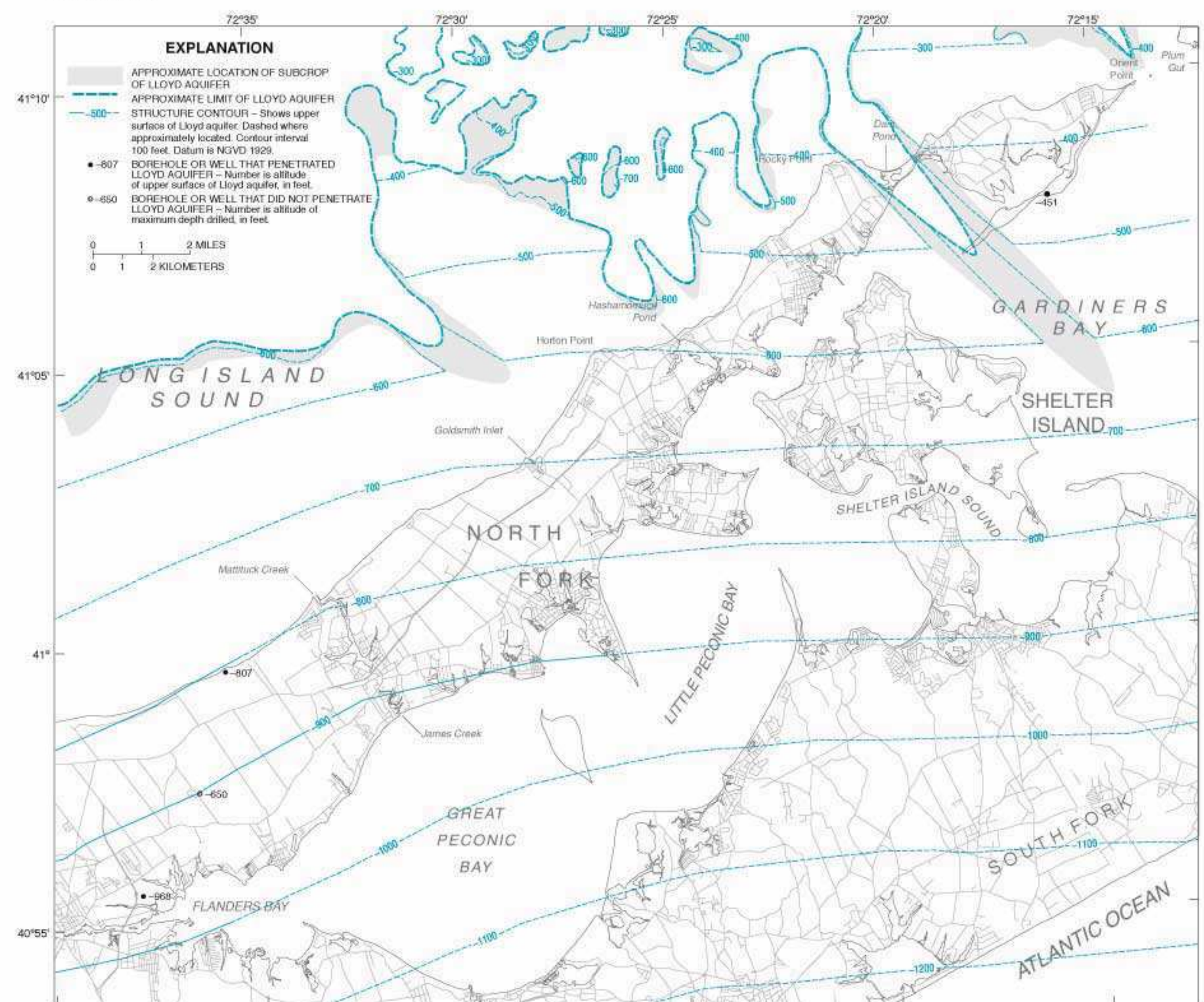
B. Lloyd aquifer
