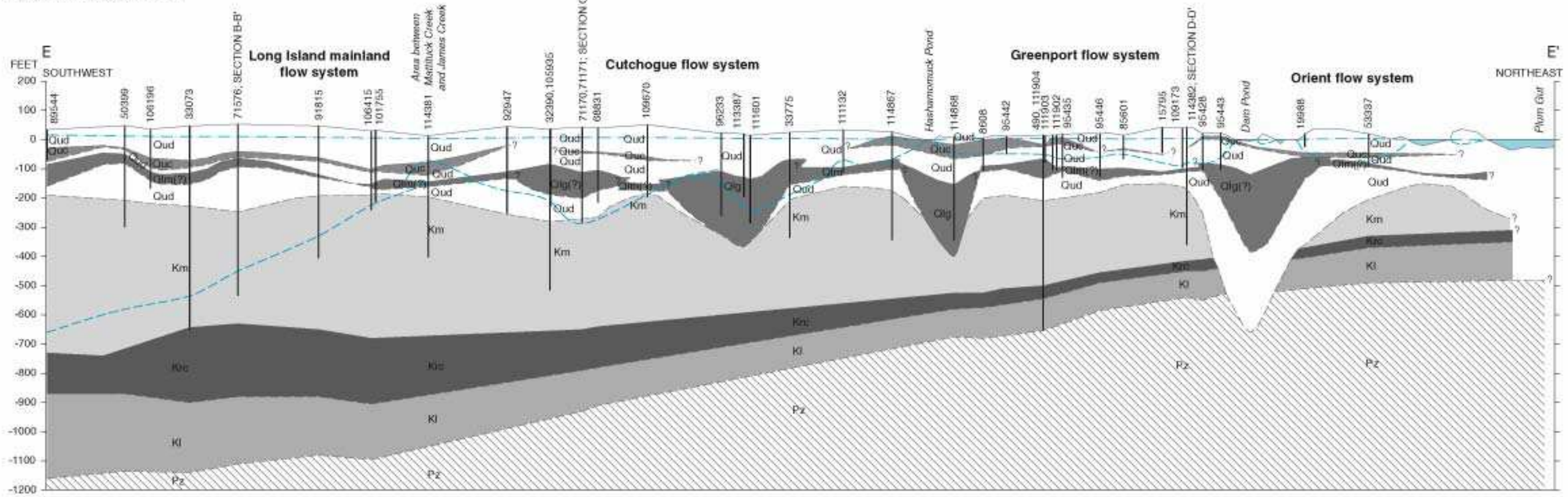
E. Vertical Section E - E'
