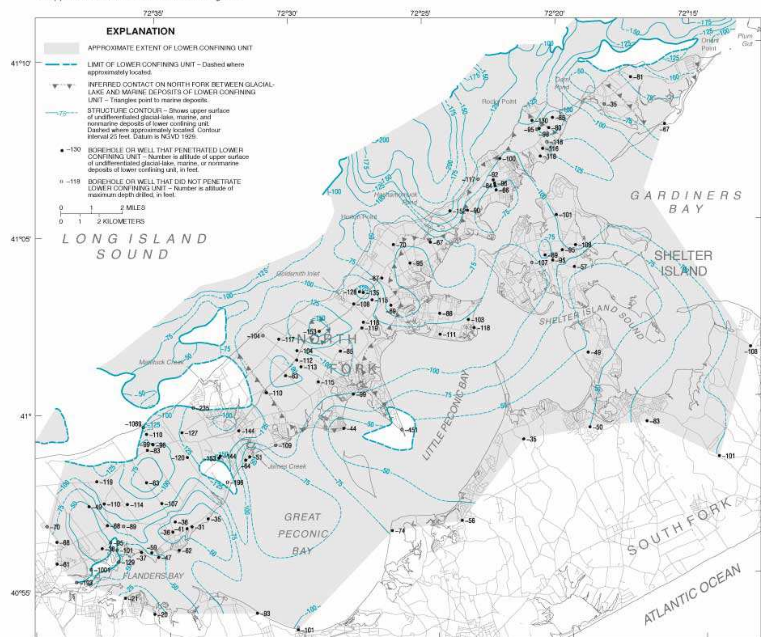
B. Upper-surface altitude of lower confining unit
